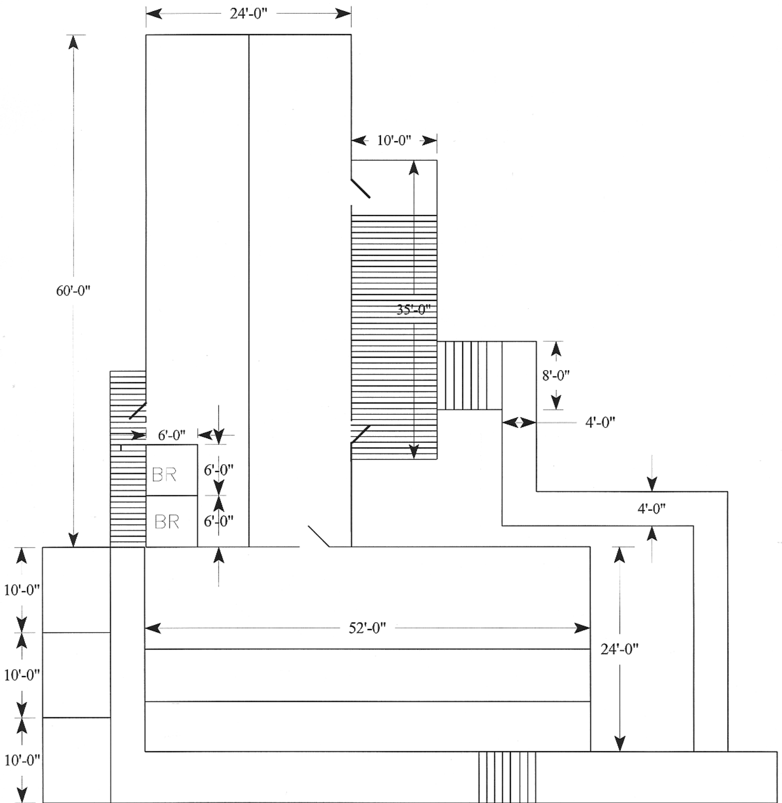
CAP BUILDING DOUBLE WIDE ADDITION
